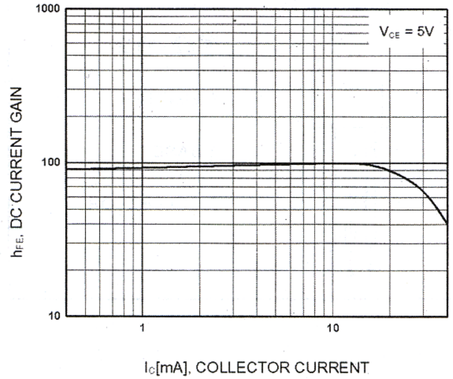
DC Current Gain
