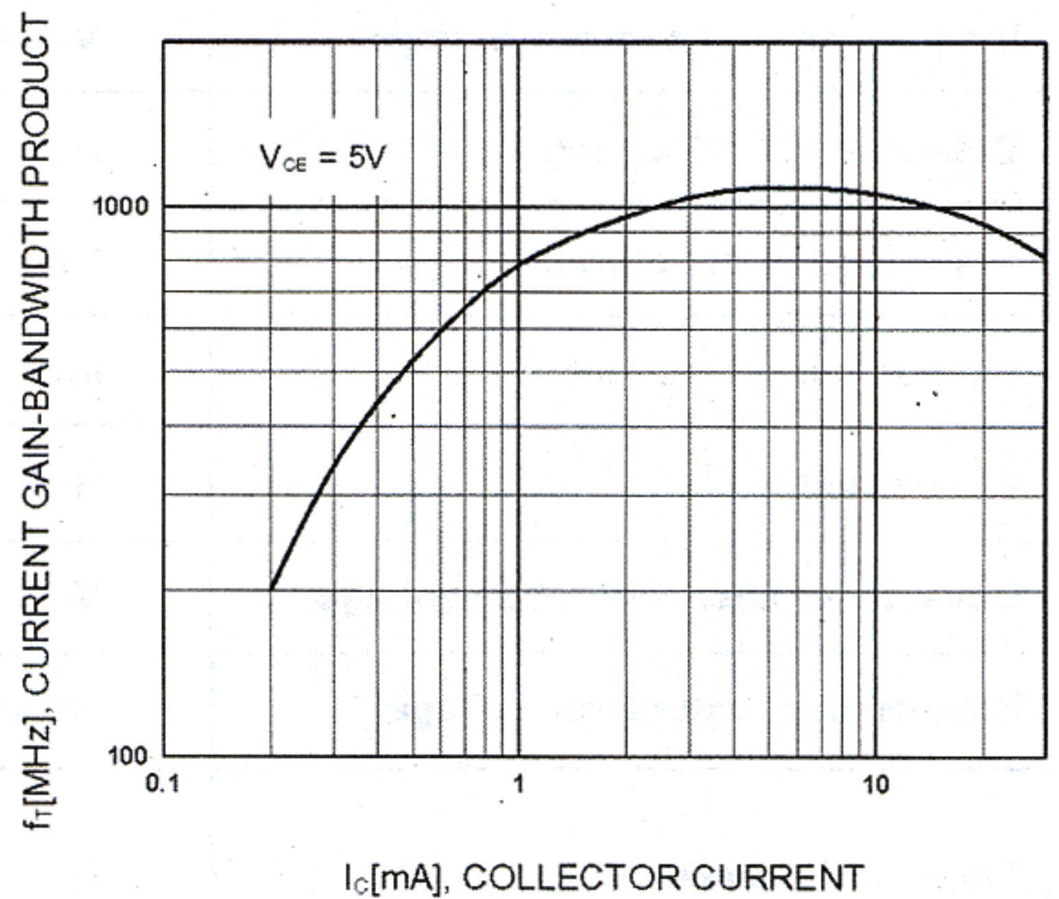
Current Gain Bandwidth Product
