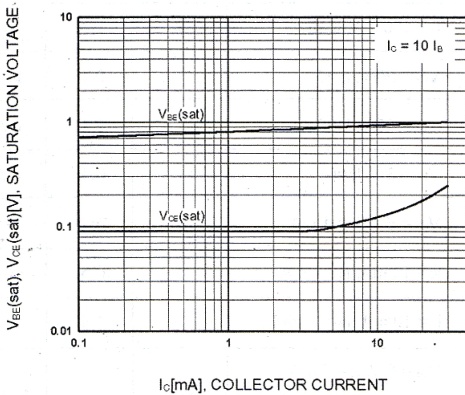
Base-Emitter Saturation Voltage Collector-Emitter Saturation Voltage
