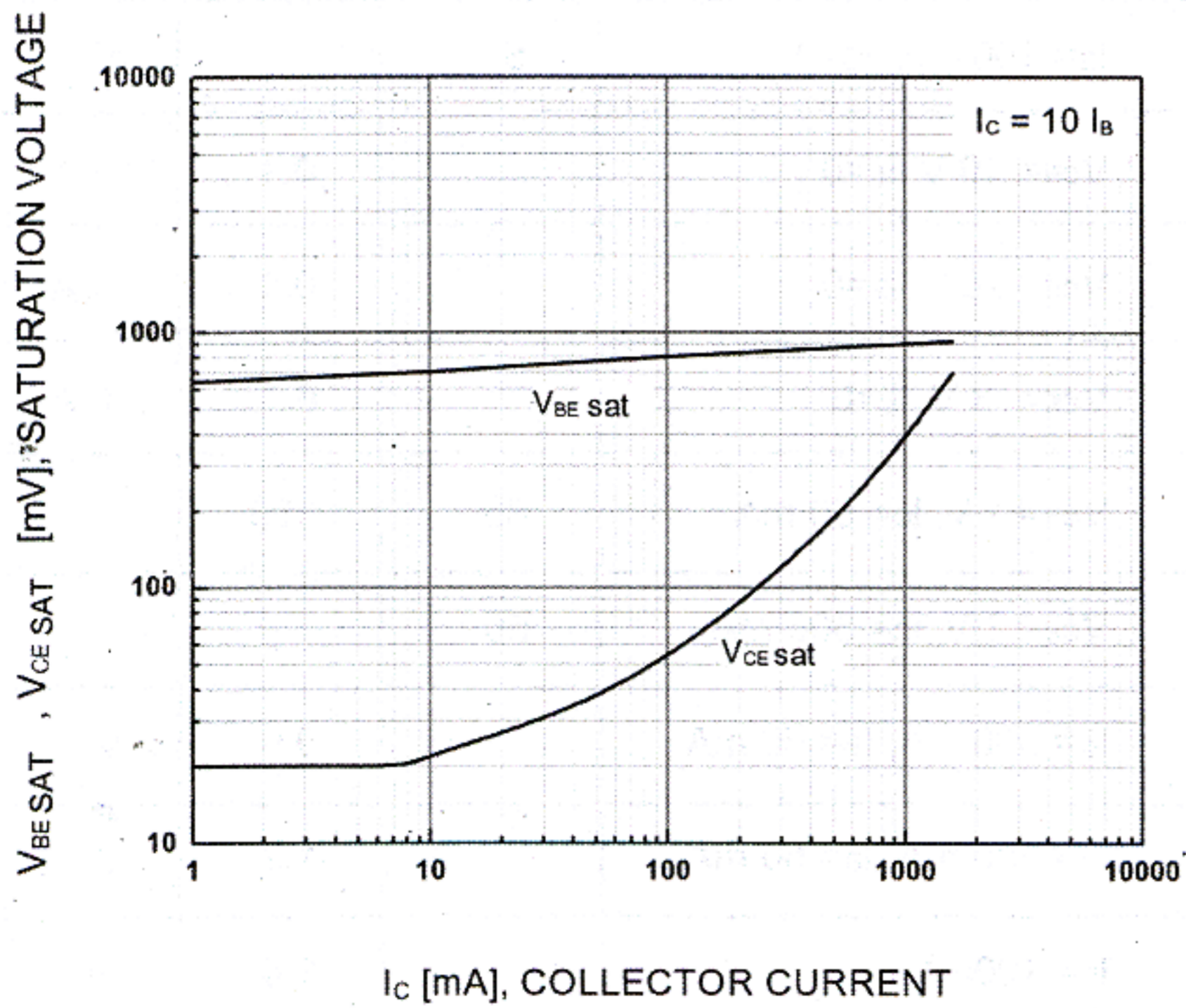
Base-Emitter Saturation Voltage Collector-Emitter Saturation Voltage
