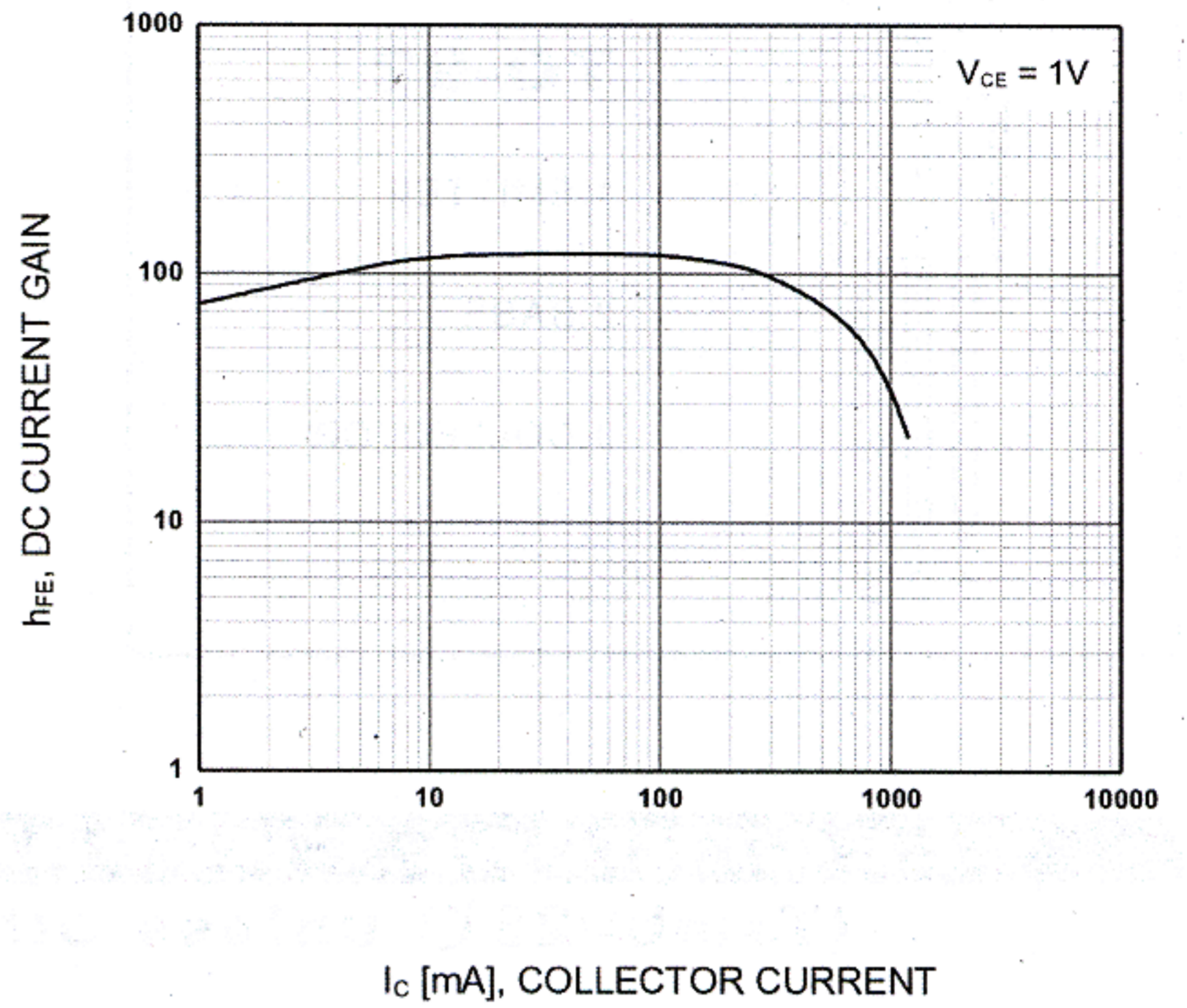
DC current Gain
