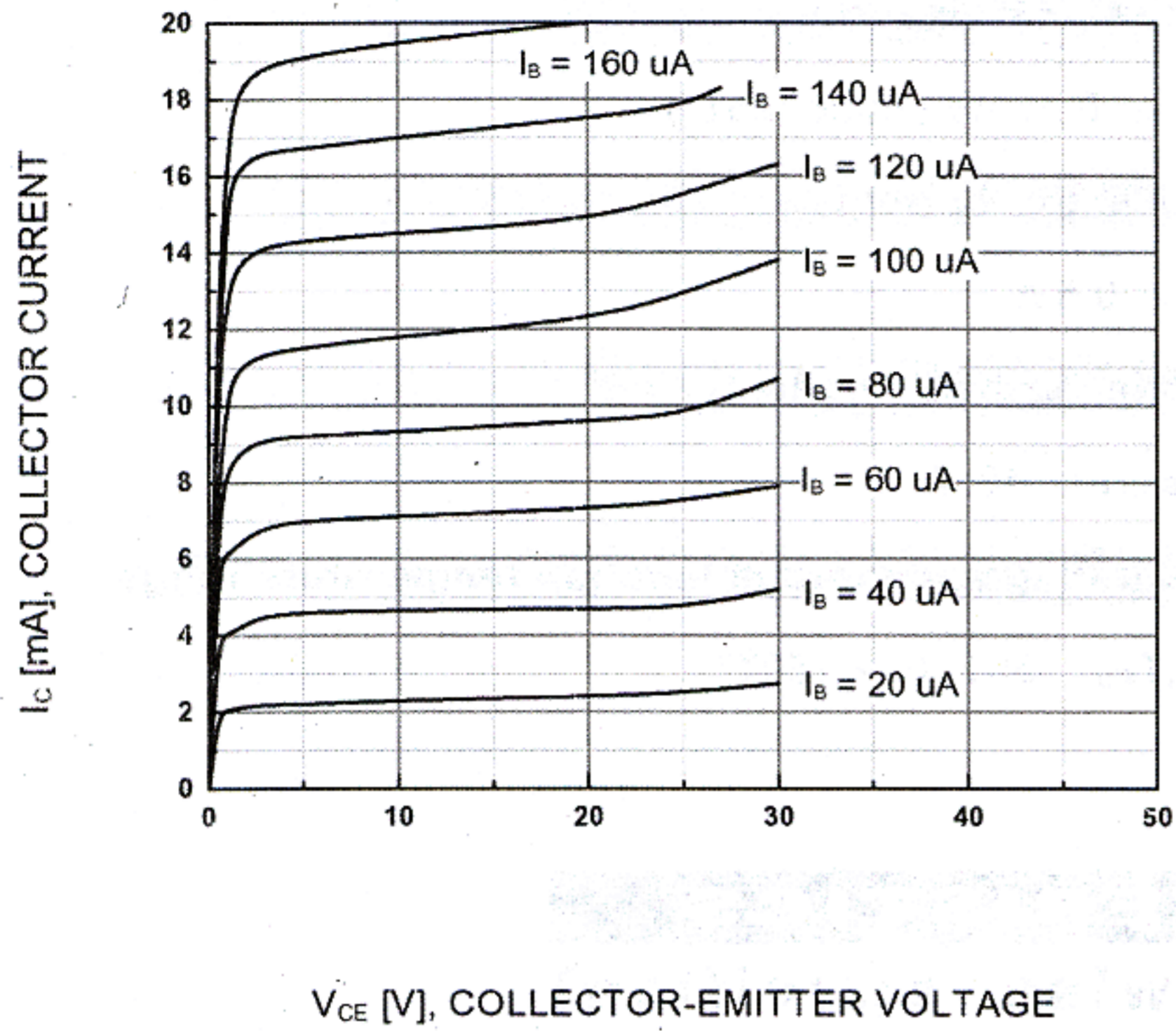
Static Characteristic
