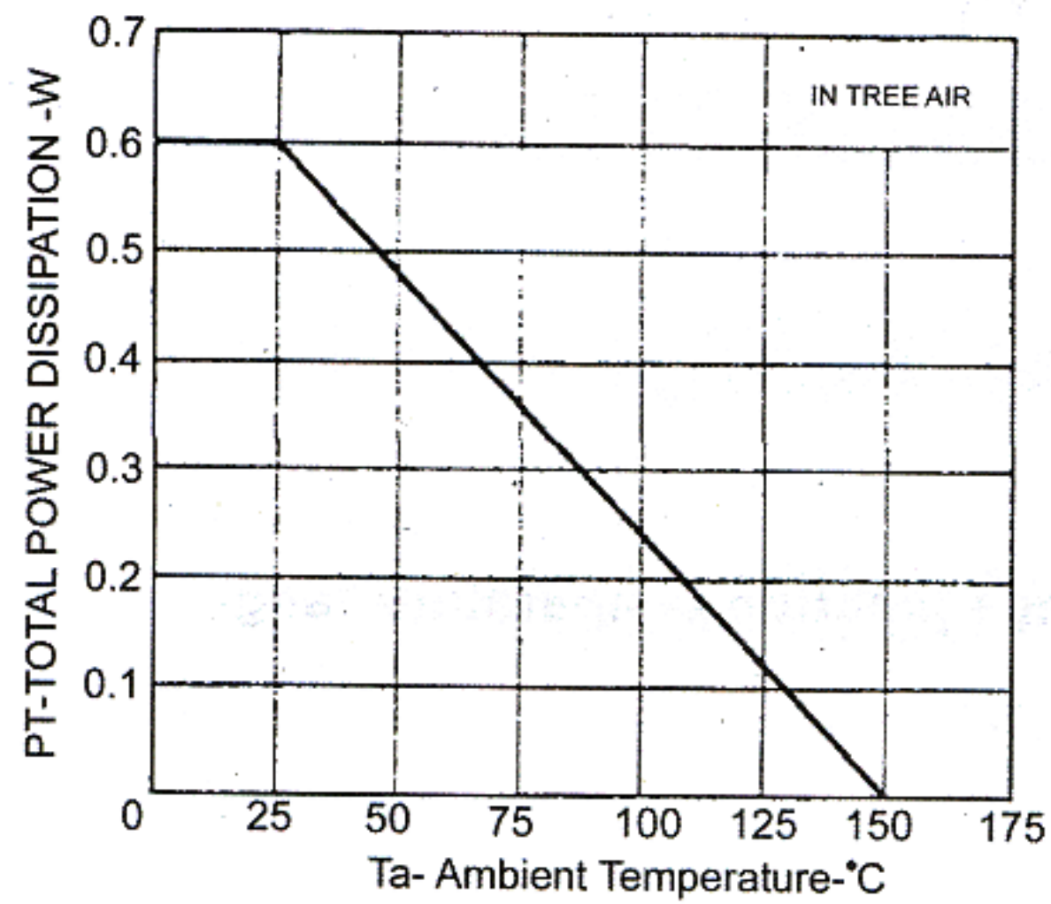
TOTAL POWER DISSIPATION VS AMBIENT TEMPERATURE
