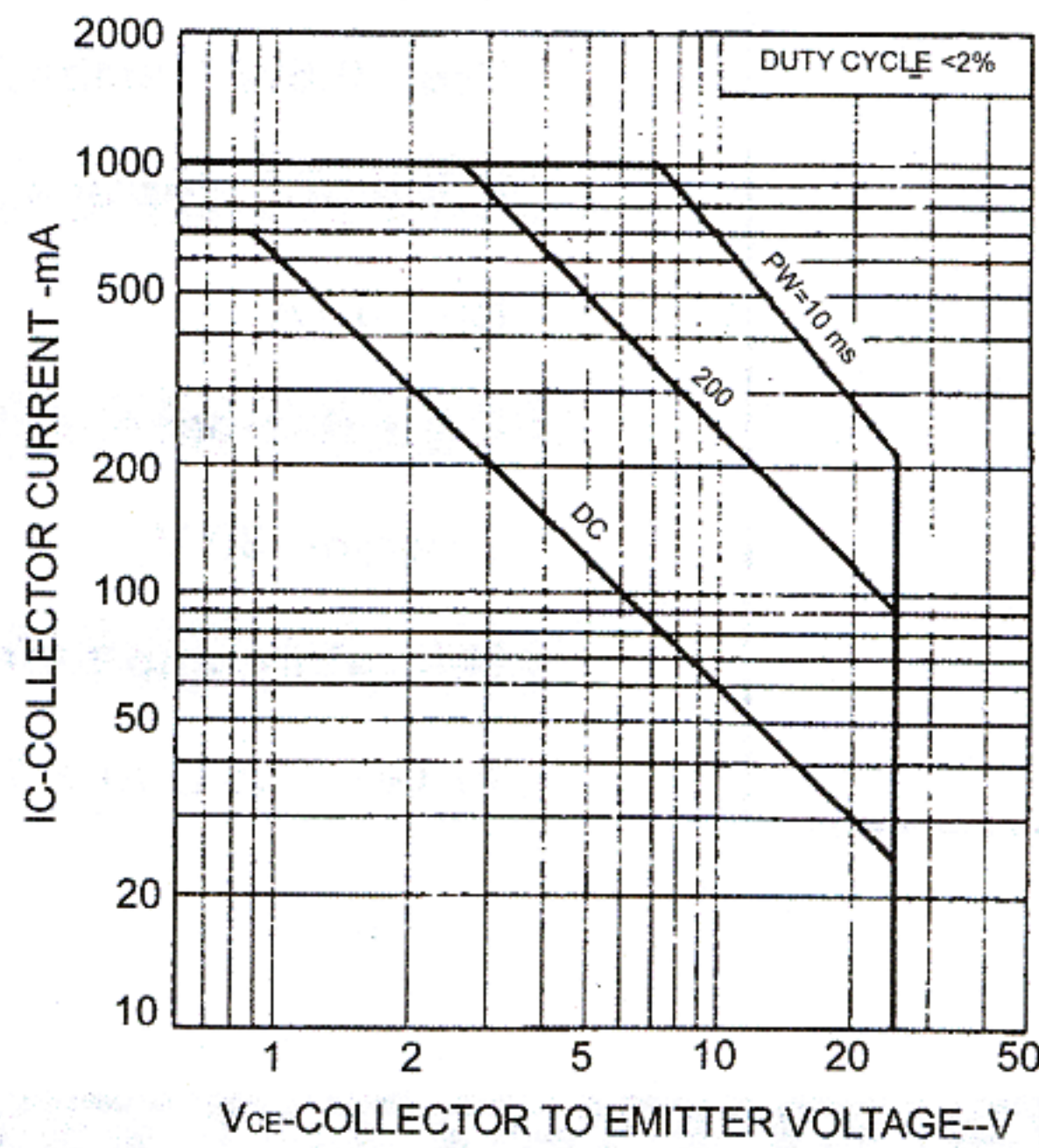
SAFE OPERATING AREA
